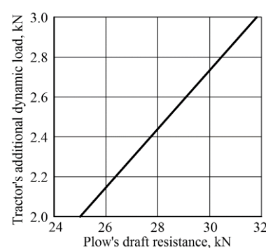
Figure 9. Tractor's additional dynamic load dependence on plough's draught resistance
