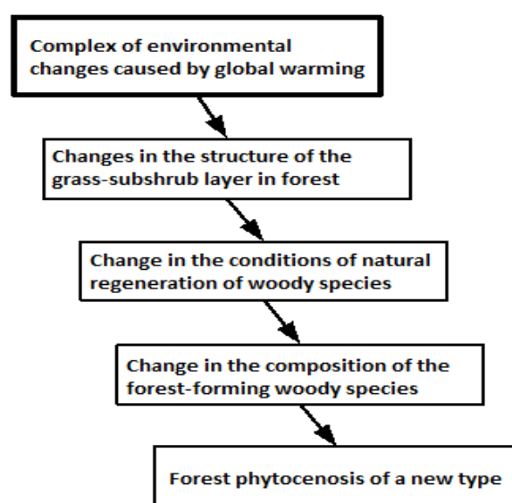
Figure 2. Diagram illustrating the chain nature of the transformation of forest ecosystems under the influence of global warming
